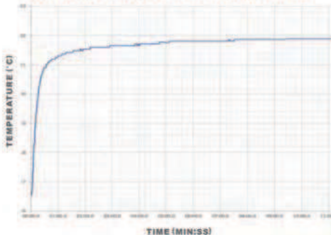
145°C ELEMENT, 1.7LPM, WATER, 700W FULL POWER RAMP TIME
